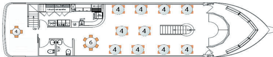
MAIN DECK ARRANGEMENT
