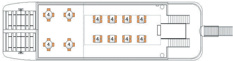
Upper Deck Arrangement
