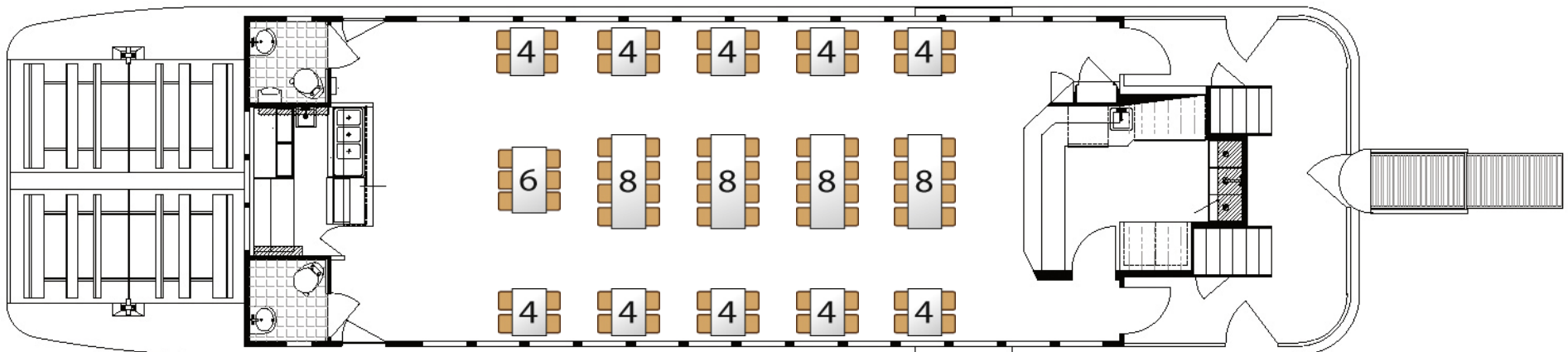
Main Deck Arrangement
