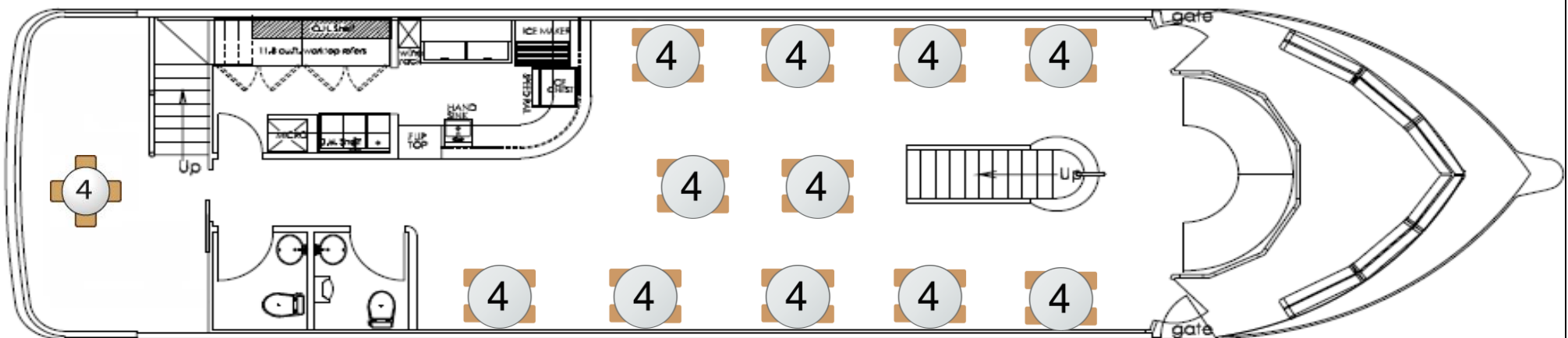
MAIN DECK ARRANGEMENT
